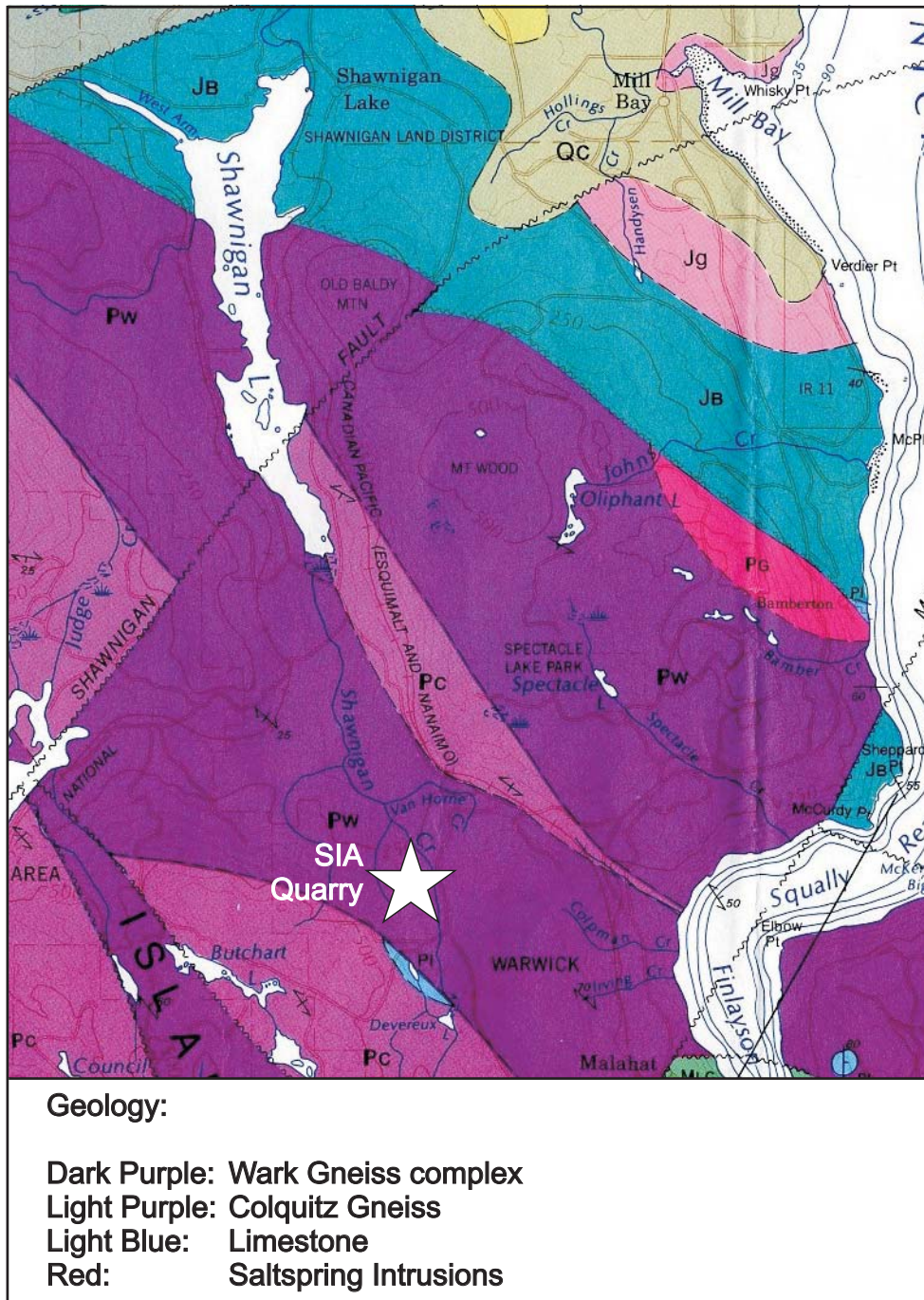
Figure 2: Map showing regional geology of the Shawnigan Lake area (modified from Muller, 1980).
